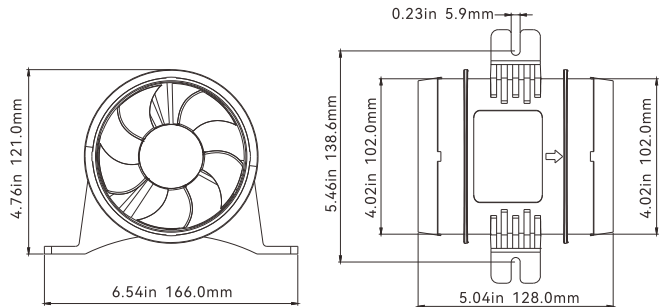
235 CFM
