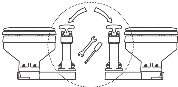
Reversible pump mounting allows left or right handed operation
